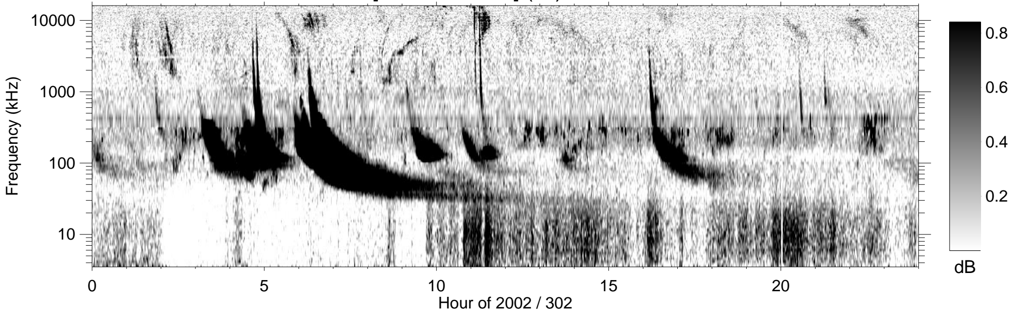
RPWS [ABCH1H2/Ex] (-B) 2002/10/29
