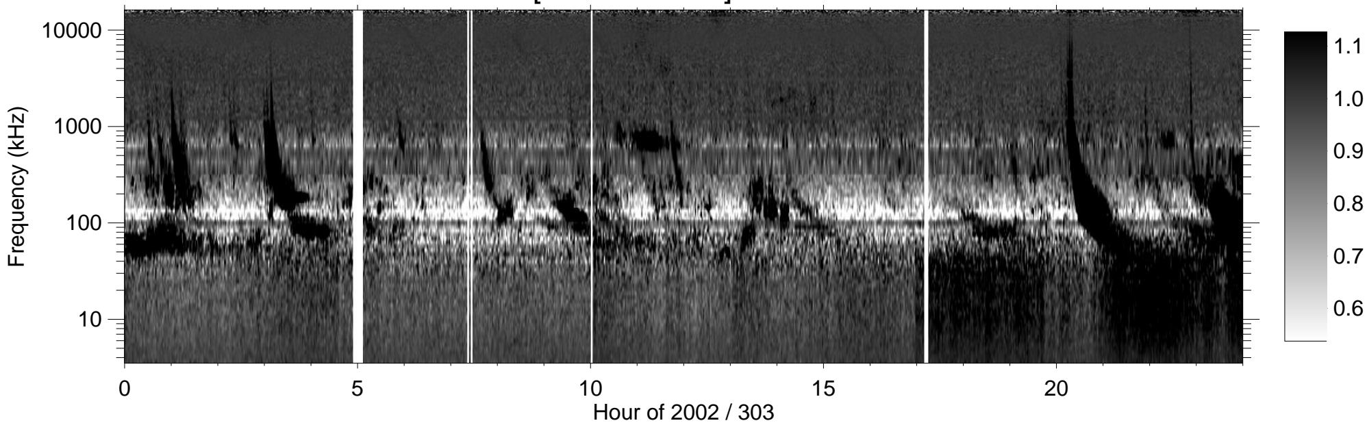
RPWS [ABCH1H2/Ex] (-B) 2002/10/30
