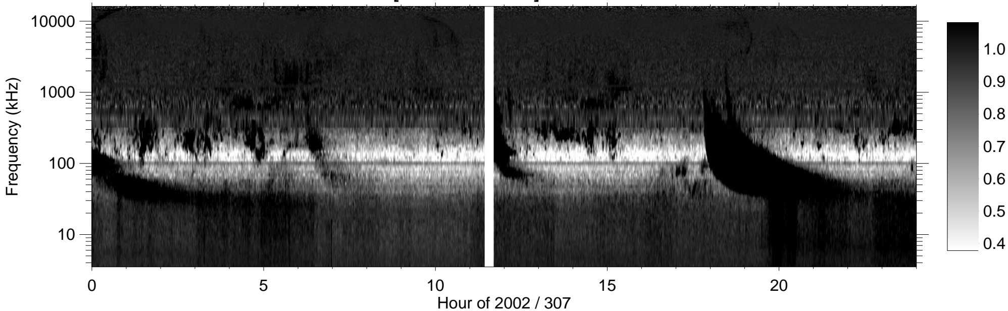
RPWS [ABCH1H2/Ex] (-B) 2002/11/03
