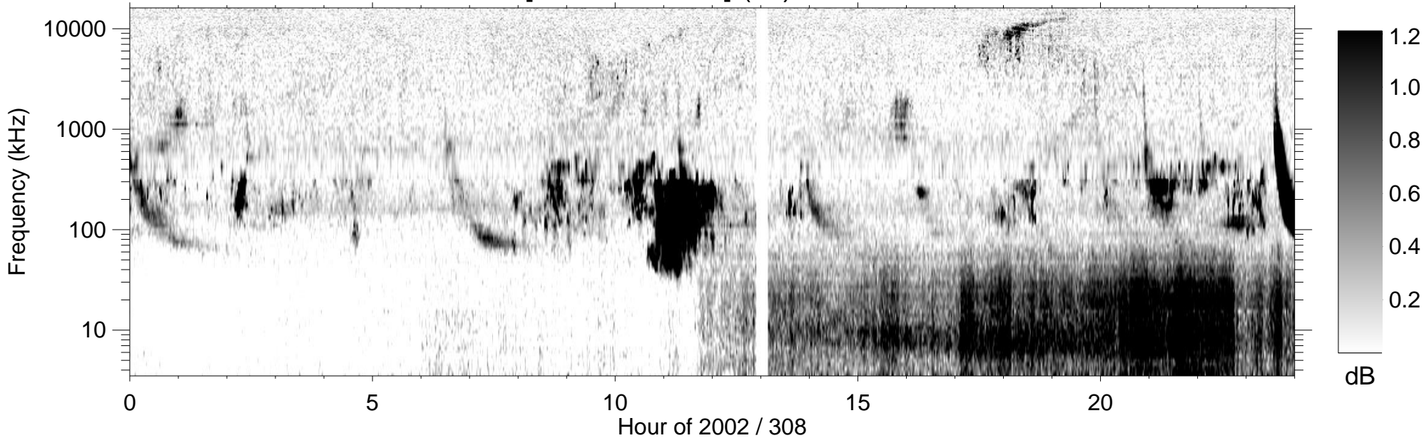
RPWS [ABCH1H2/Ex] (-B) 2002/11/04
