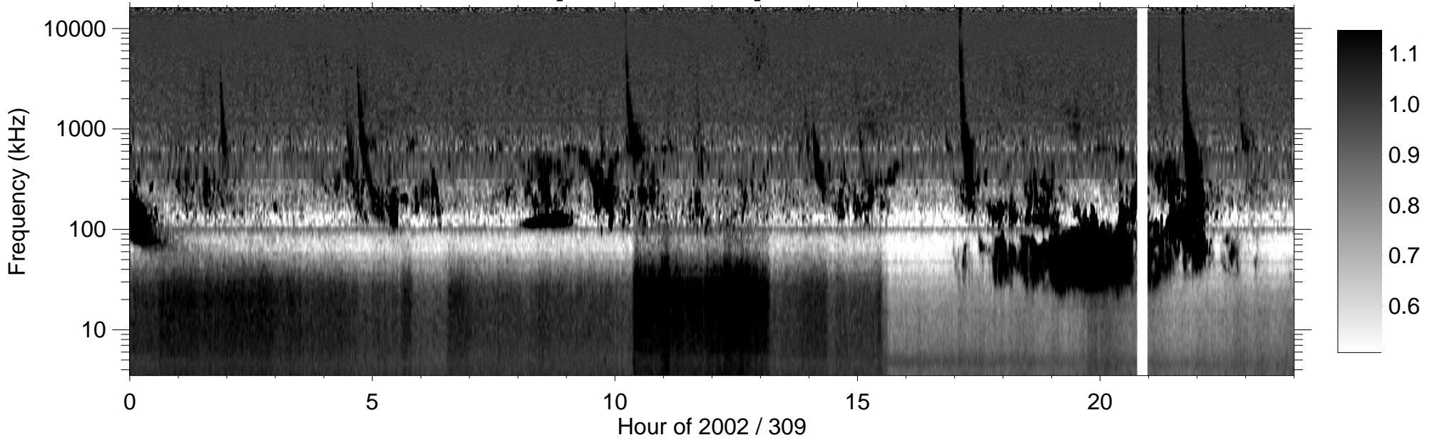
RPWS [ABCH1H2/Ex] (-B) 2002/11/05
