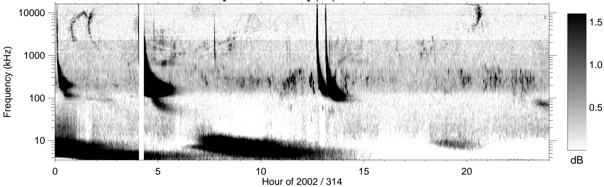
RPWS [ABCH1H2/Ex] (-B) 2002/11/10
