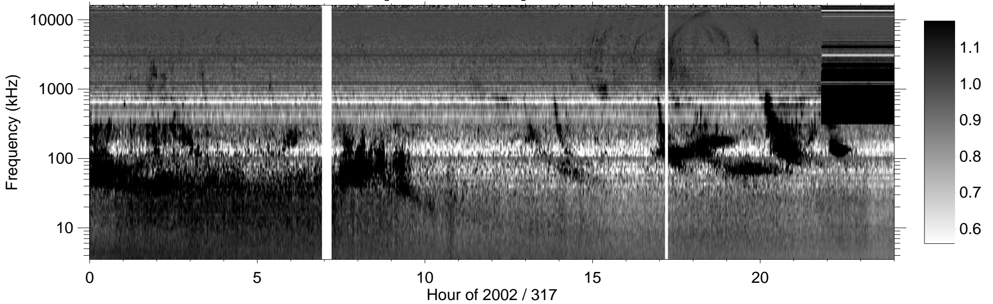
RPWS [ABCH1H2/Ex] (-B) 2002/11/13
