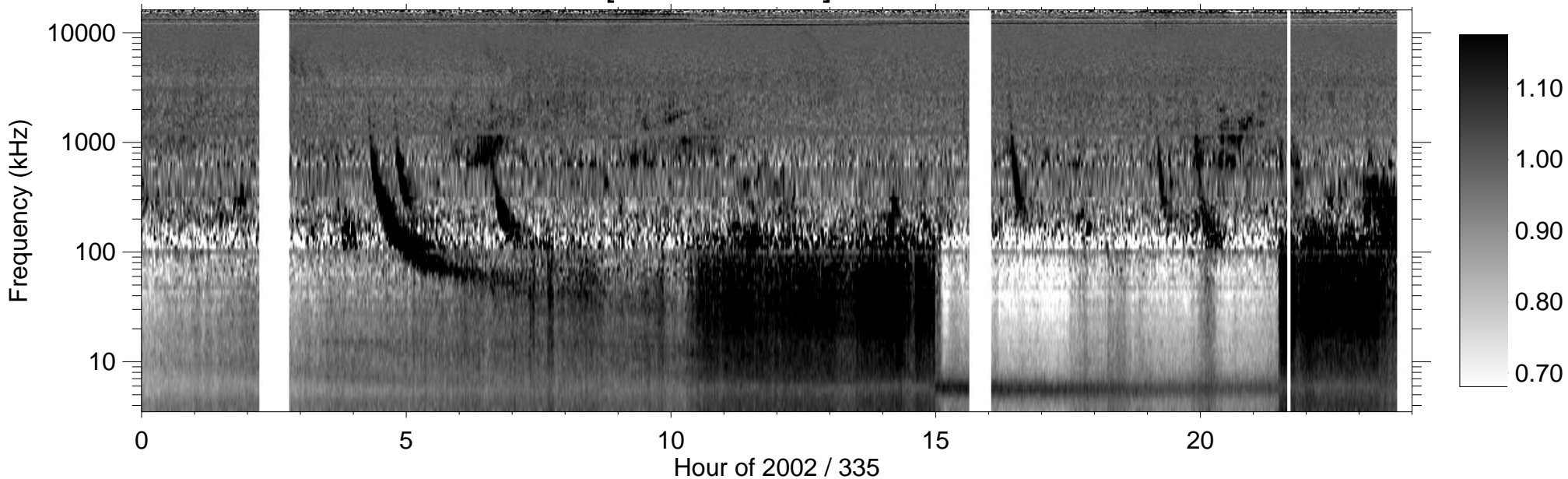
RPWS [ABCH1H2/Ex] (-B) 2002/12/01
