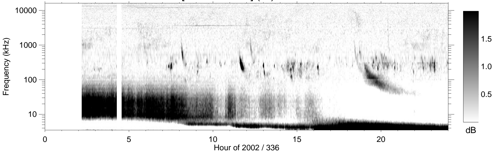
RPWS [ABCH1H2/Ex] (-B) 2002/12/02
