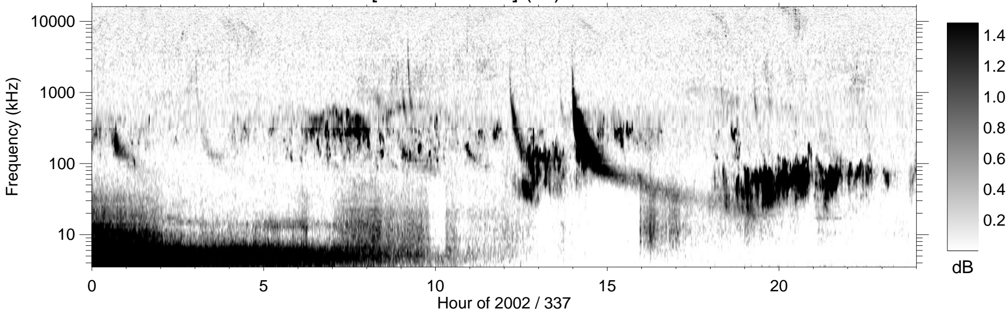
RPWS [ABCH1H2/Ex] (-B) 2002/12/03
