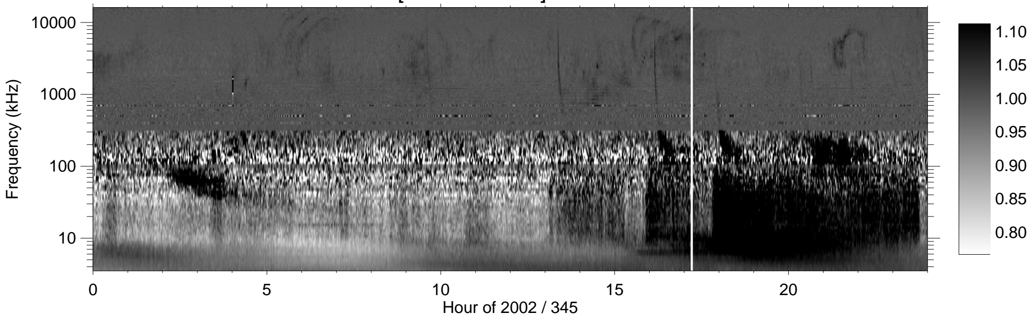
RPWS [ABCH1H2/Ex] (-B) 2002/12/11
