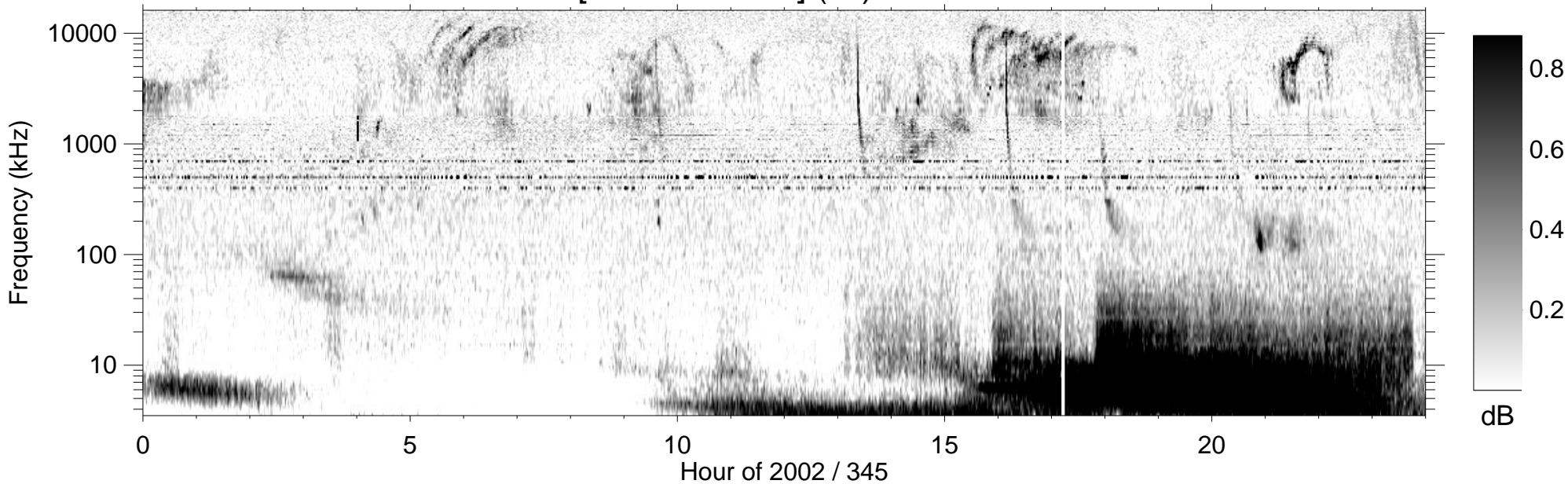
RPWS [ABCH1H2/Ex] (-B) 2002/12/11
