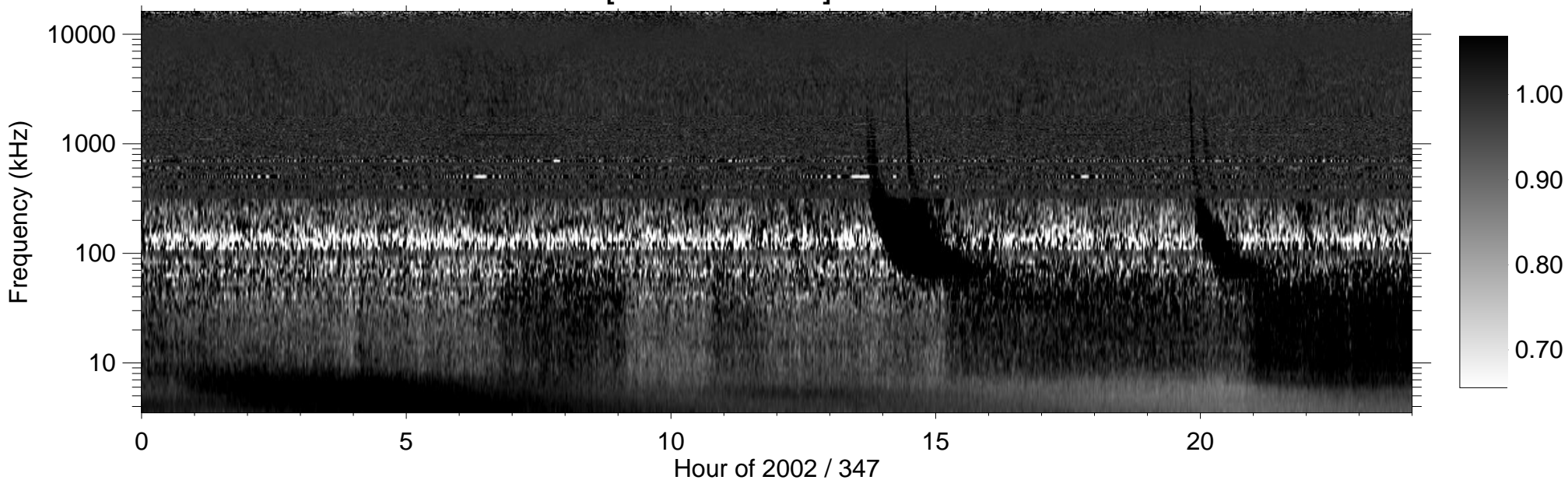
RPWS [ABCH1H2/Ex] (-B) 2002/12/13
