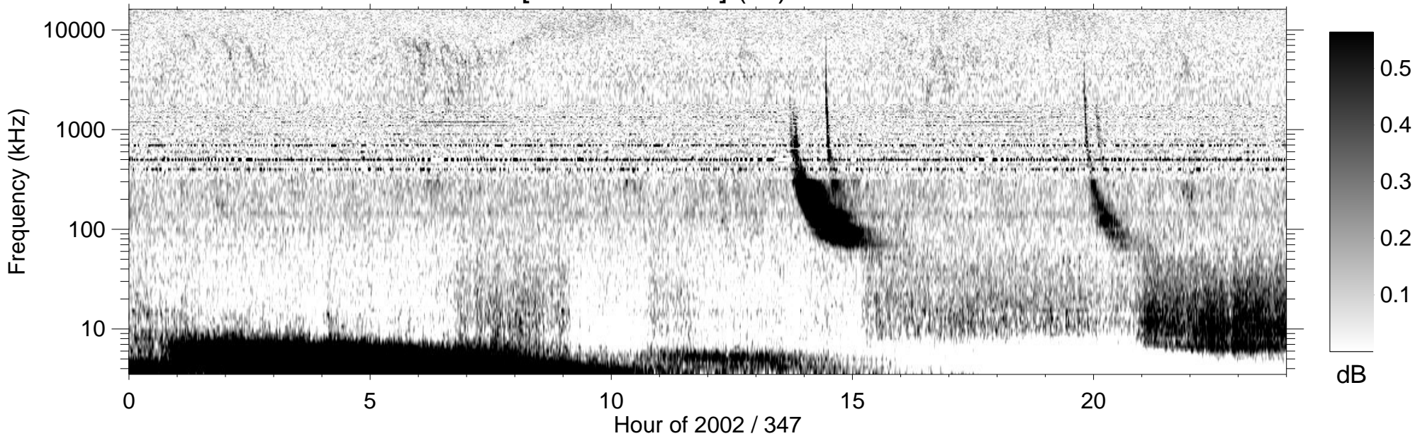
RPWS [ABCH1H2/Ex] (-B) 2002/12/13
