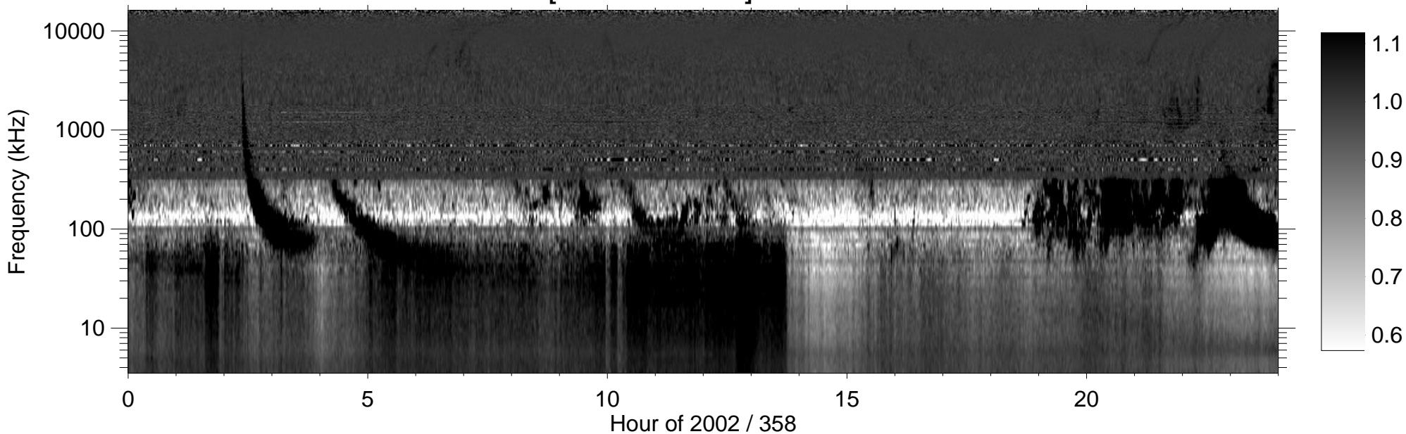
RPWS [ABCH1H2/Ex] (-B) 2002/12/24
