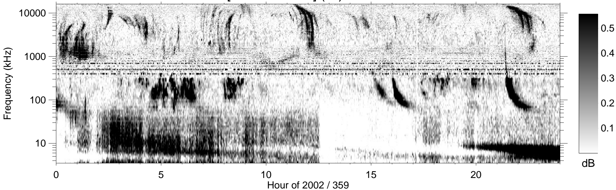
RPWS [ABCH1H2/Ex] (-B) 2002/12/25
