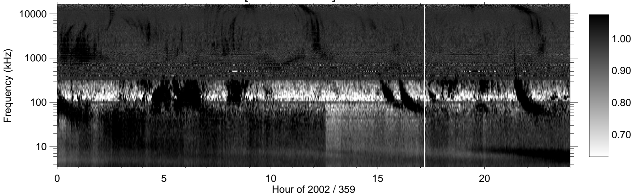
RPWS [ABCH1H2/Ex] (-B) 2002/12/25
