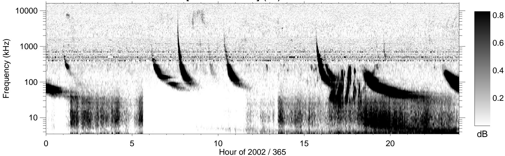
RPWS [ABCH1H2/Ex] (-B) 2002/12/31
