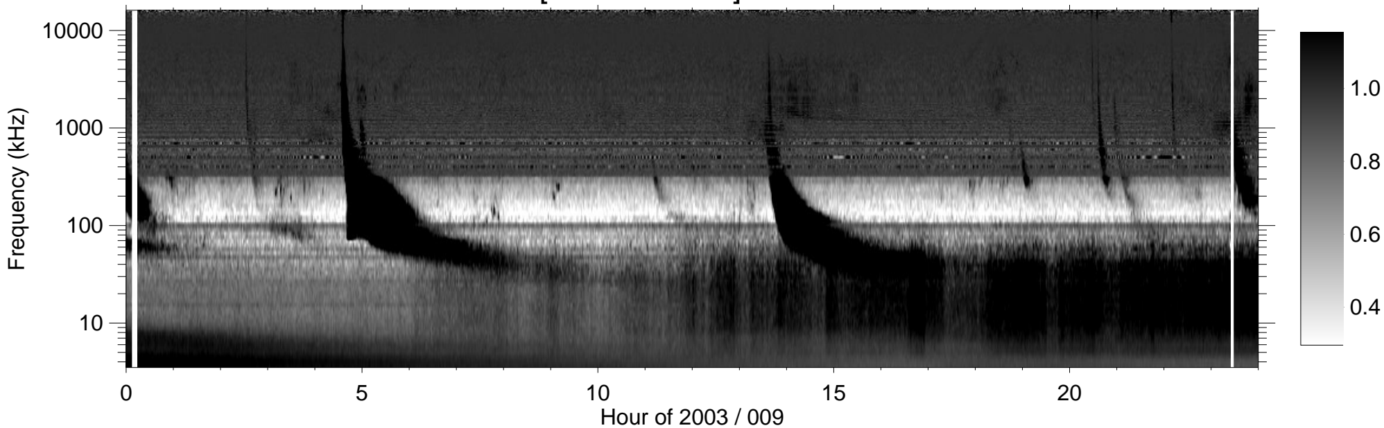
RPWS [ABCH1H2/Ex] (-B) 2003/01/09
