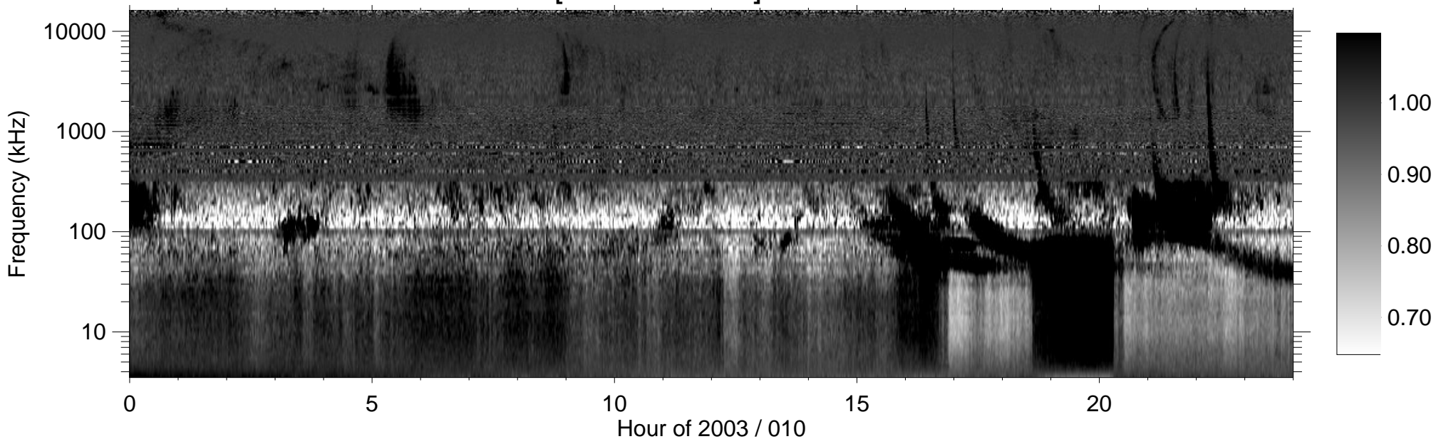
RPWS [ABCH1H2/Ex] (-B) 2003/01/10
