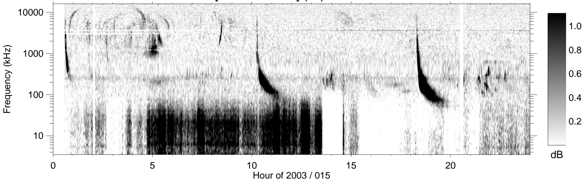
RPWS [ABCH1H2/Ex] (-B) 2003/01/15
