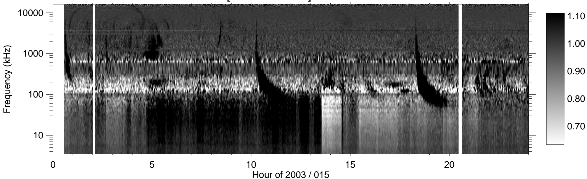
RPWS [ABCH1H2/Ex] (-B) 2003/01/15
