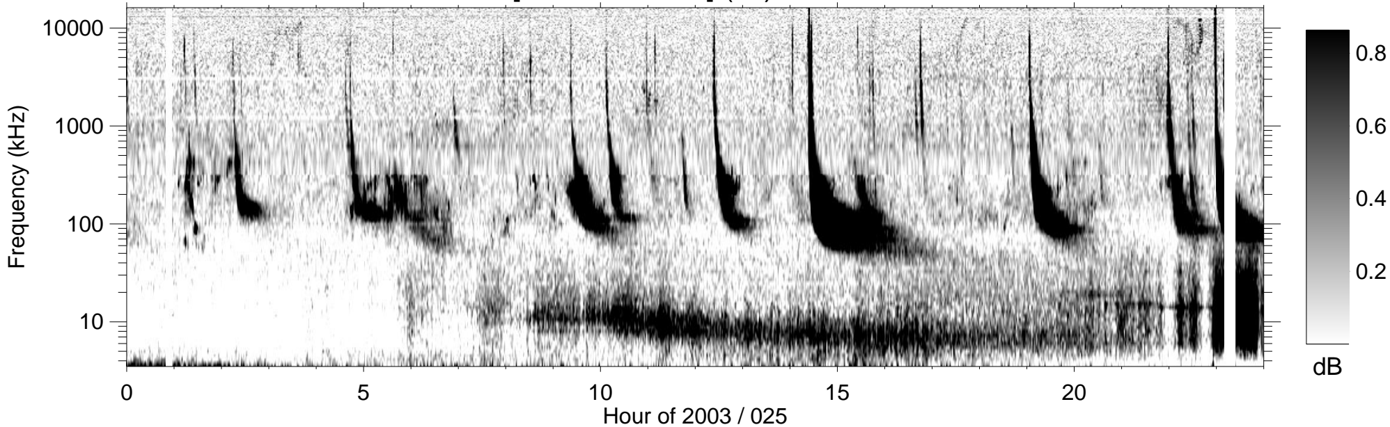
RPWS [ABCH1H2/Ex] (-B) 2003/01/25
