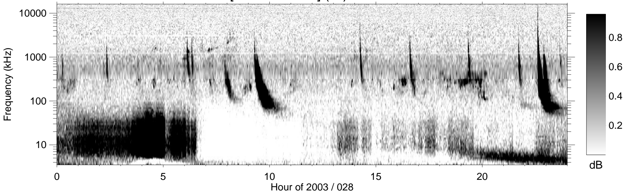
RPWS [ABCH1H2/Ex] (-B) 2003/01/28
