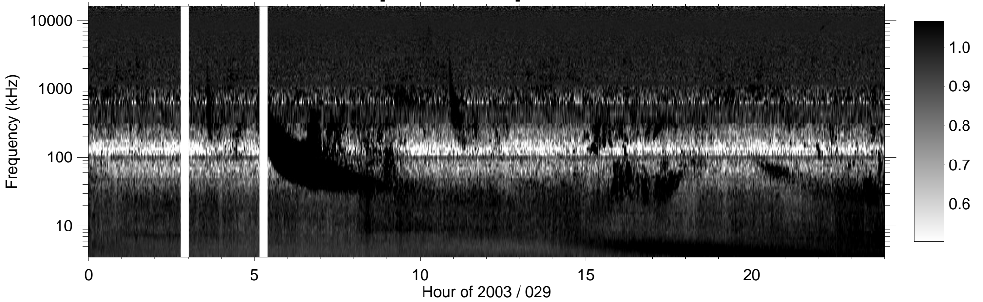
RPWS [ABCH1H2/Ex] (-B) 2003/01/29
