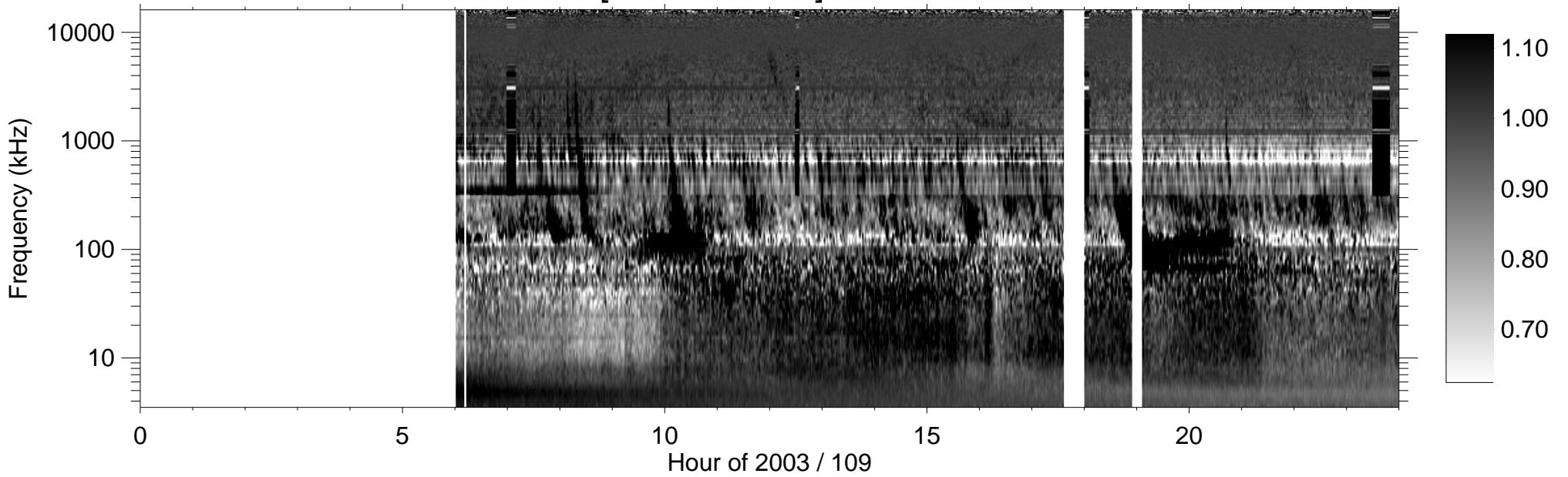
RPWS [ABCH1H2/Ex] (-B) 2003/04/19
