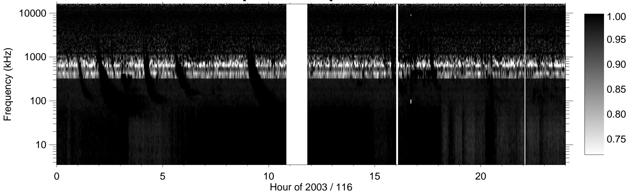
RPWS [ABCH1H2/Ex] (-B) 2003/04/26
