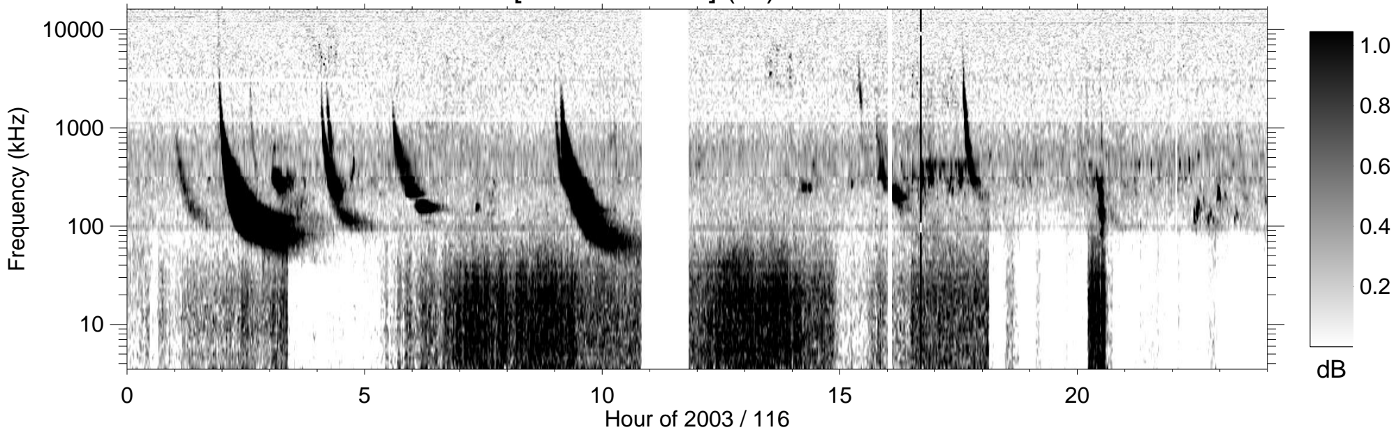
RPWS [ABCH1H2/Ex] (-B) 2003/04/26
