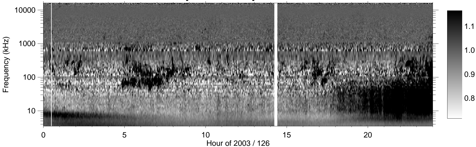
RPWS [ABCH1H2/Ex] (-B) 2003/05/06
