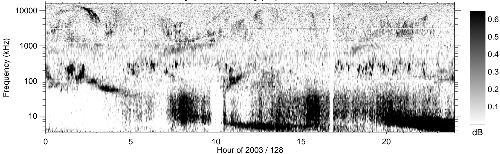
RPWS [ABCH1H2/Ex] (-B) 2003/05/08
