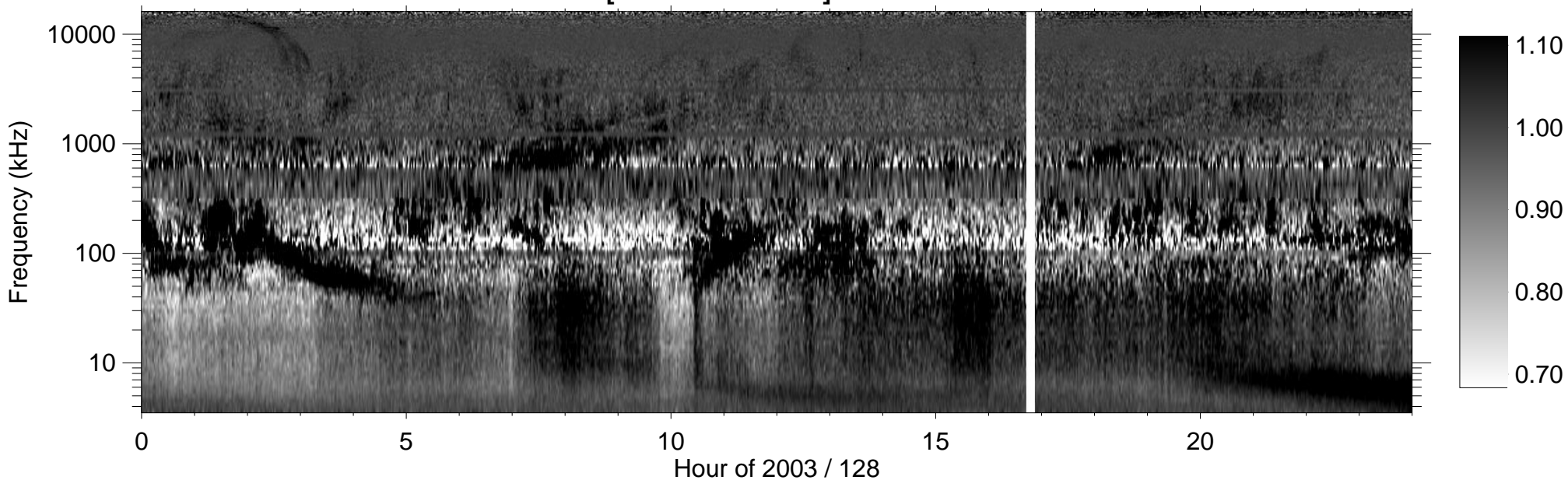
RPWS [ABCH1H2/Ex] (-B) 2003/05/08
