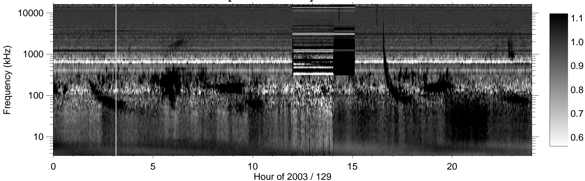
RPWS [ABCH1H2/Ex] (-B) 2003/05/09
