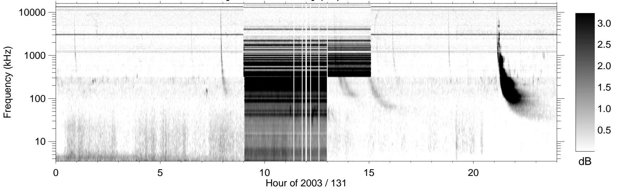
RPWS [ABCH1H2/Ex] (-B) 2003/05/11
