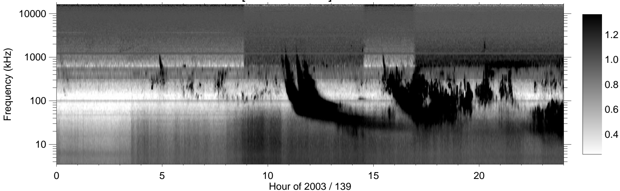
RPWS [ABCH1H2/Ex] (-B) 2003/05/19
