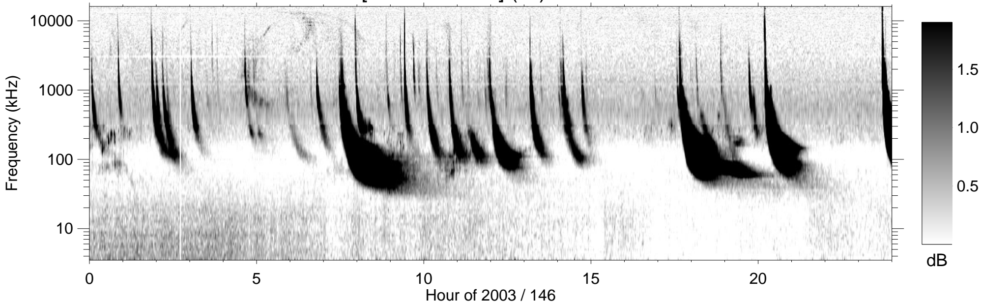
RPWS [ABCH1H2/Ex] (-B) 2003/05/26
