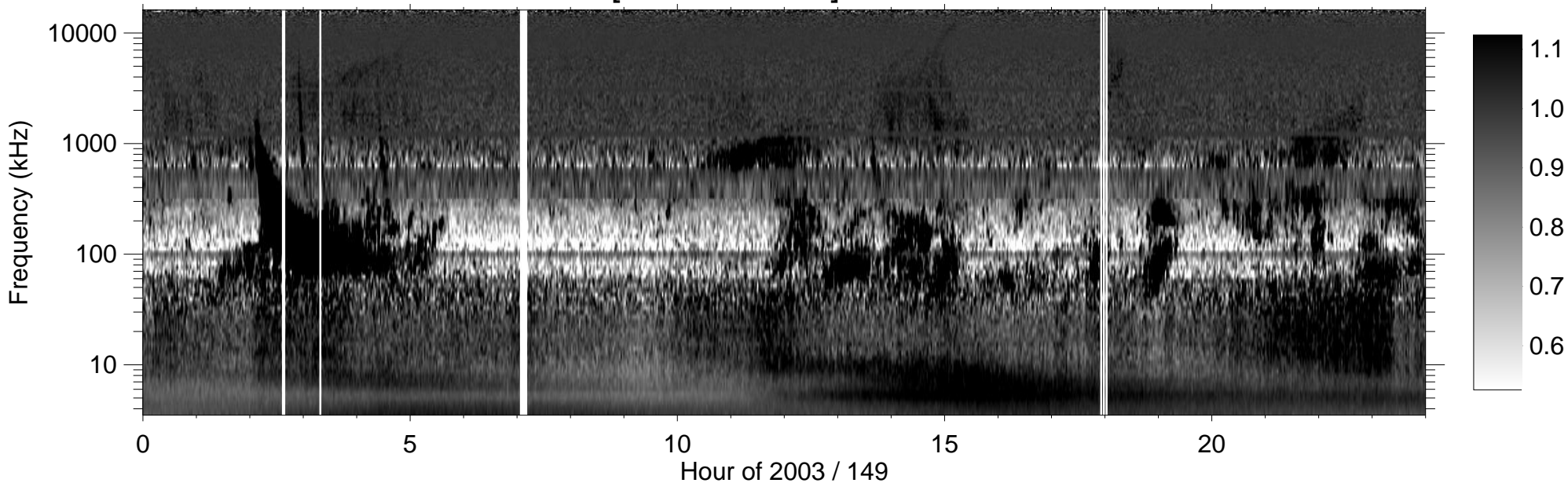
RPWS [ABCH1H2/Ex] (-B) 2003/05/29
