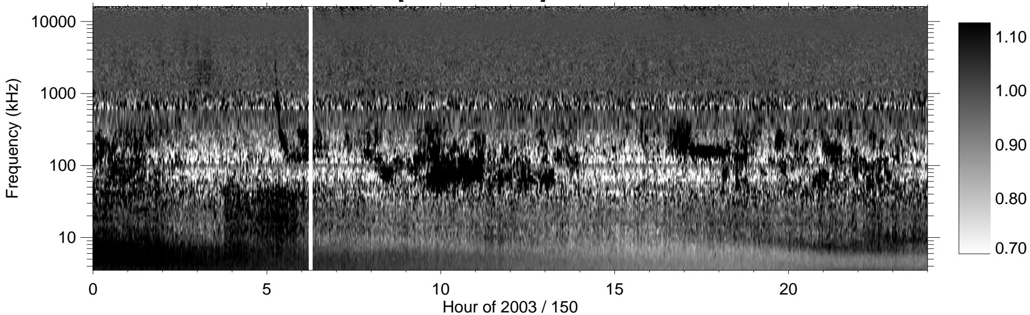
RPWS [ABCH1H2/Ex] (-B) 2003/05/30
