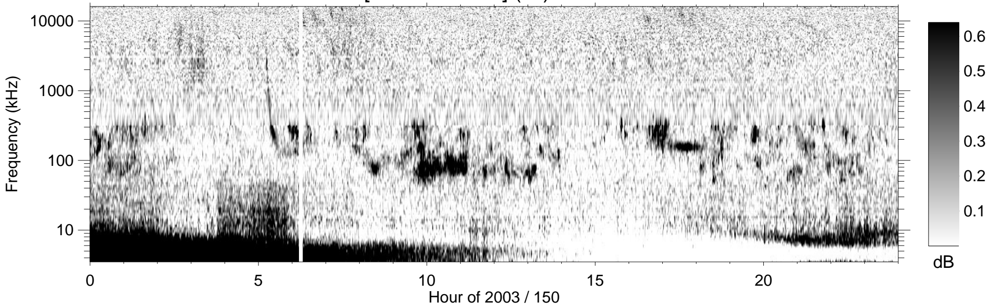
RPWS [ABCH1H2/Ex] (-B) 2003/05/30
