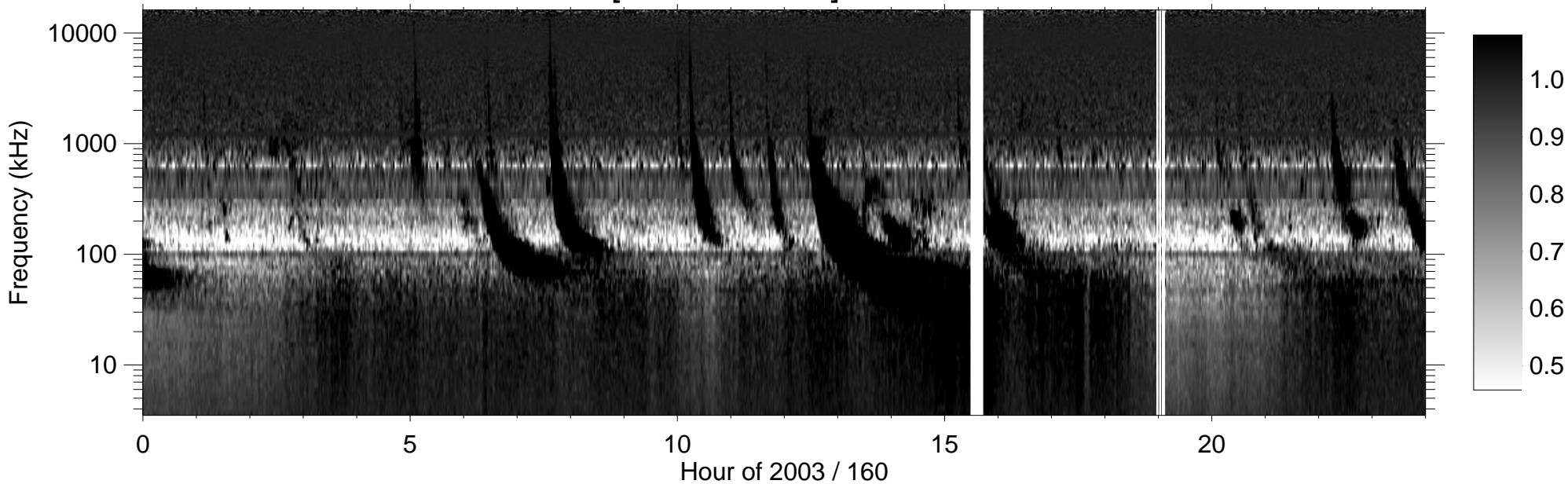
RPWS [ABCH1H2/Ex] (-B) 2003/06/09
