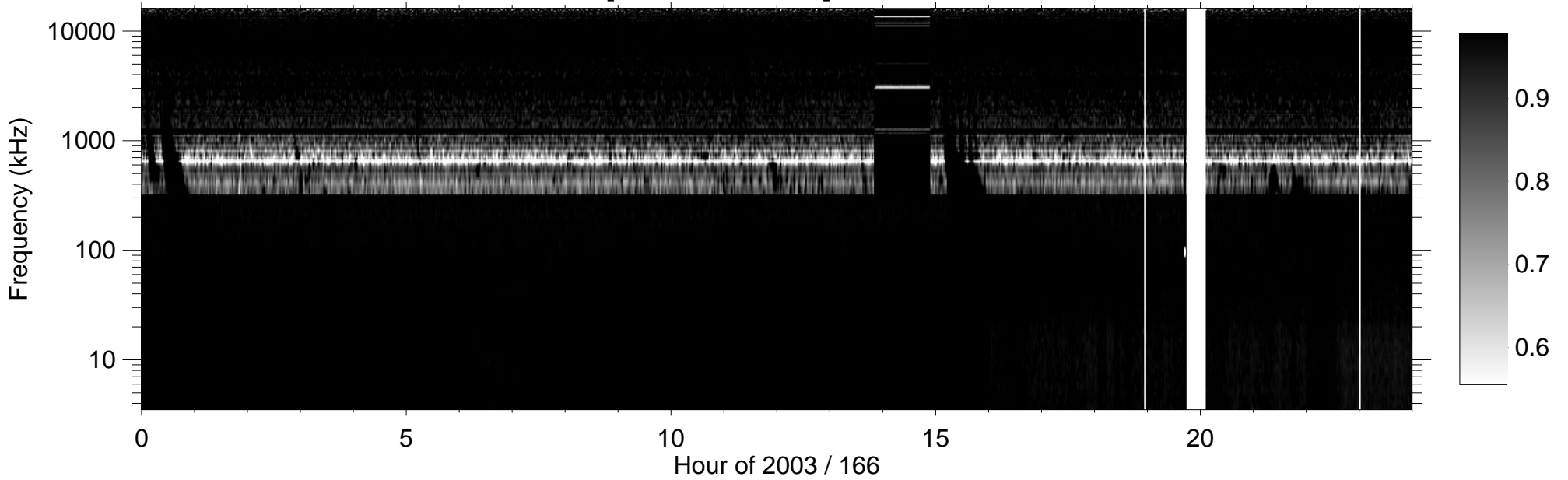
RPWS [ABCH1H2/Ex] (-B) 2003/06/15
