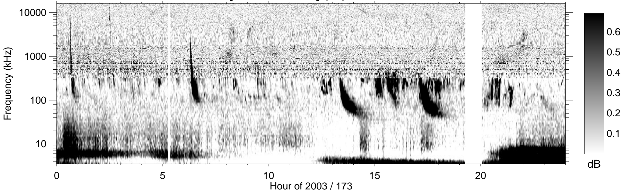
RPWS [ABCH1H2/Ex] (-B) 2003/06/22
