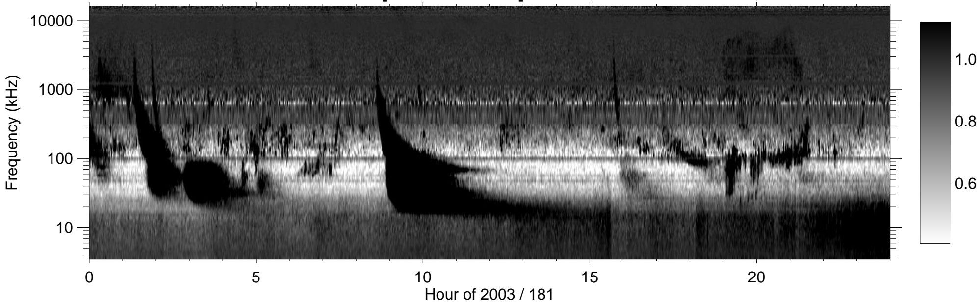
RPWS [ABCH1H2/Ex] (-B) 2003/06/30
