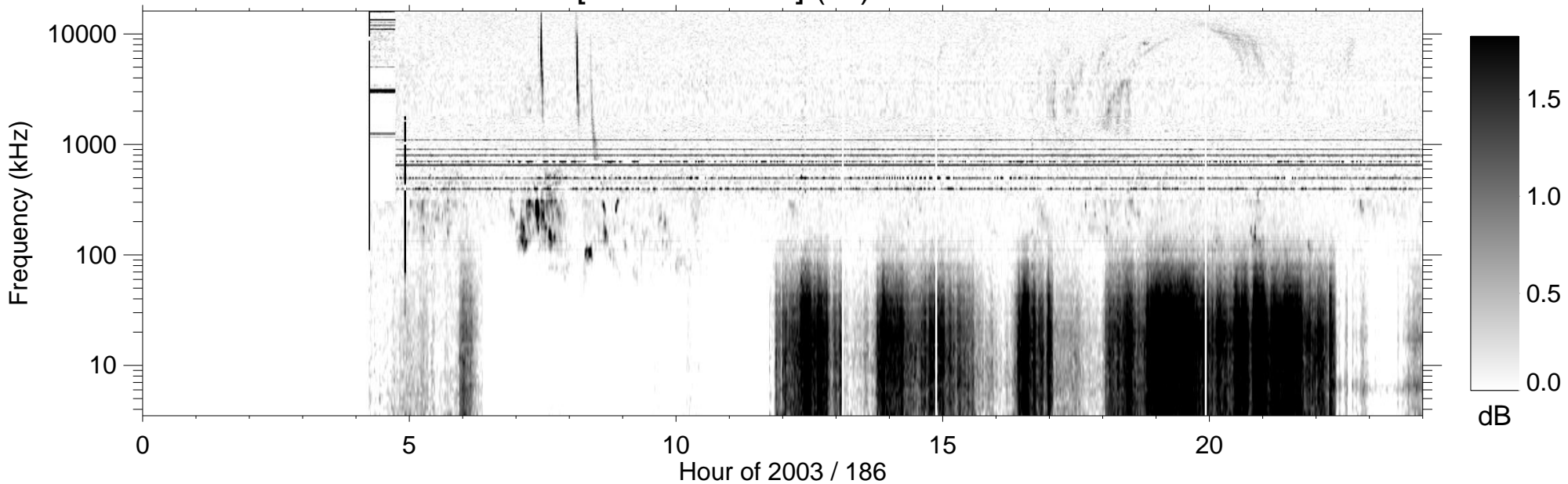
RPWS [ABCH1H2/Ex] (-B) 2003/07/05
