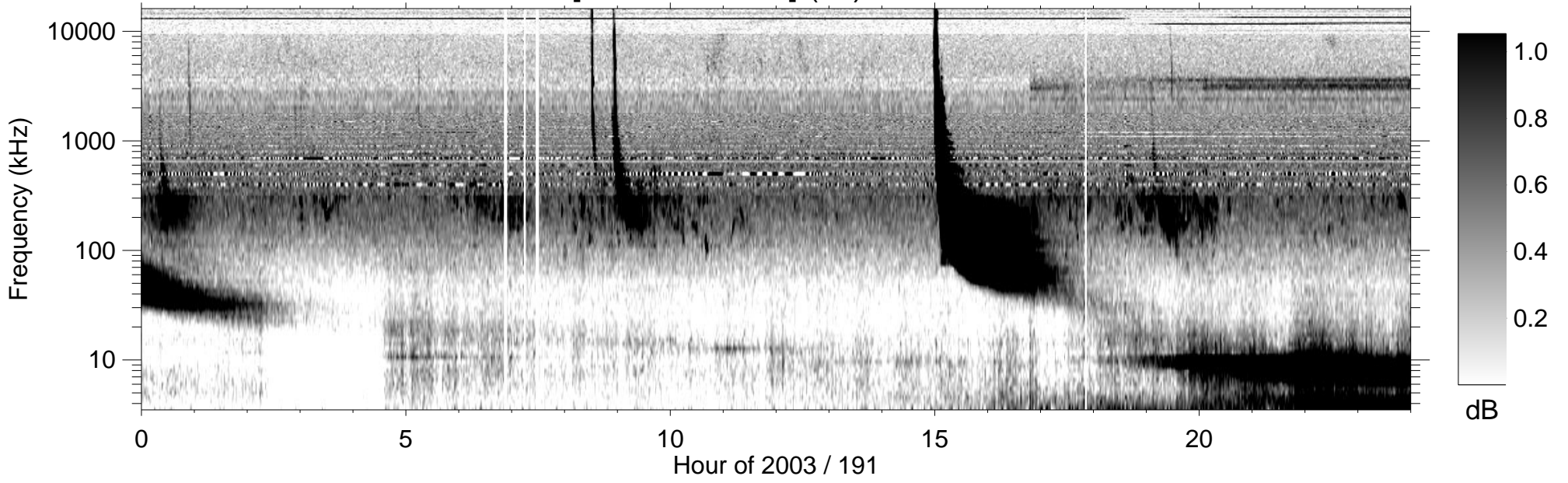
RPWS [ABCH1H2/Ex] (-B) 2003/07/10
