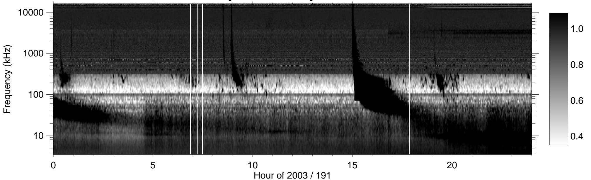
RPWS [ABCH1H2/Ex] (-B) 2003/07/10
