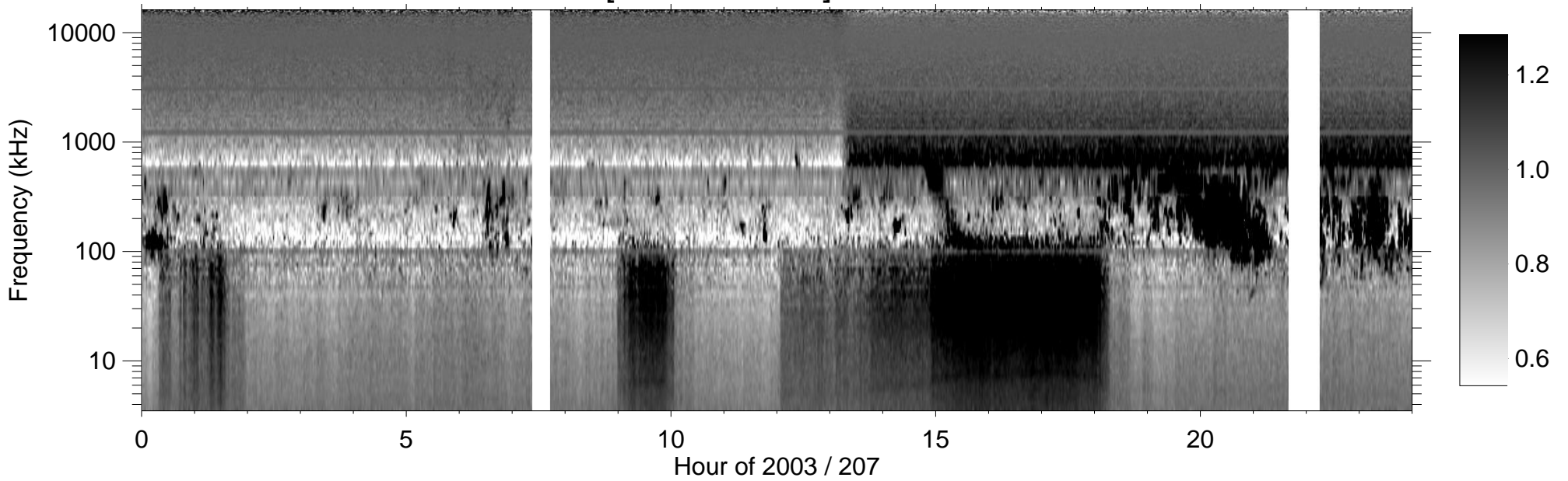
RPWS [ABCH1H2/Ex] (-B) 2003/07/26
