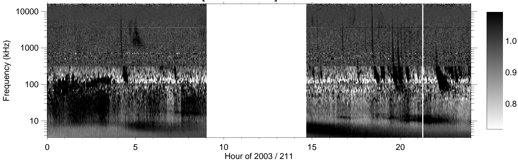
RPWS [ABCH1H2/Ex] (-B) 2003/07/30
