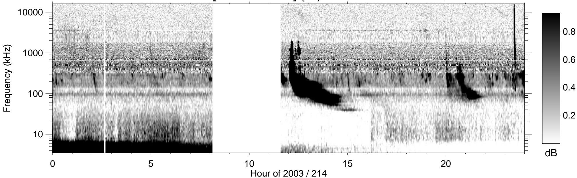
RPWS [ABCH1H2/Ex] (-B) 2003/08/02
