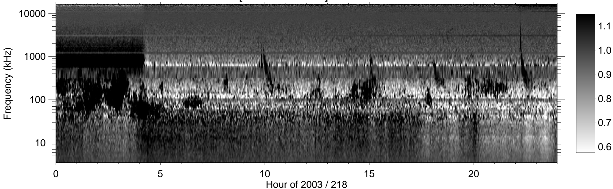
RPWS [ABCH1H2/Ex] (-B) 2003/08/06
