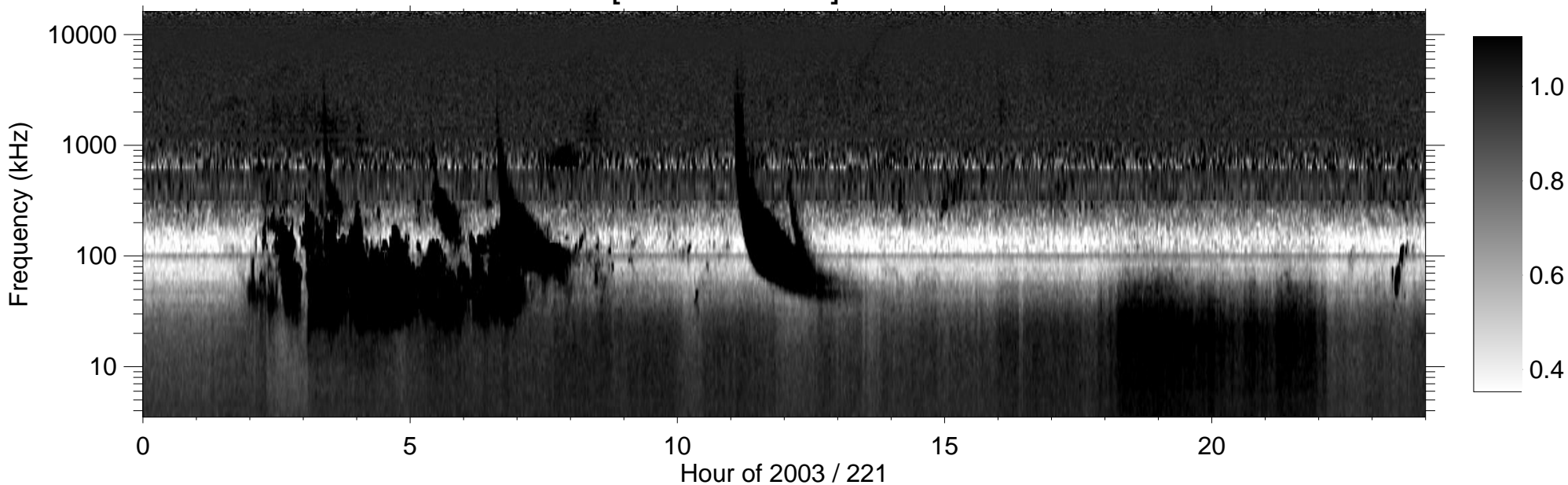
RPWS [ABCH1H2/Ex] (-B) 2003/08/09
