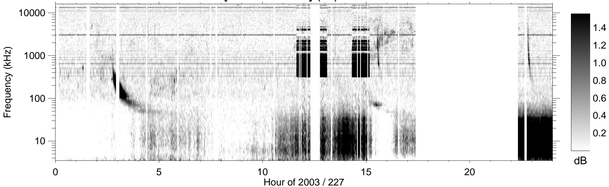
RPWS [ABCH1H2/Ex] (-B) 2003/08/15
