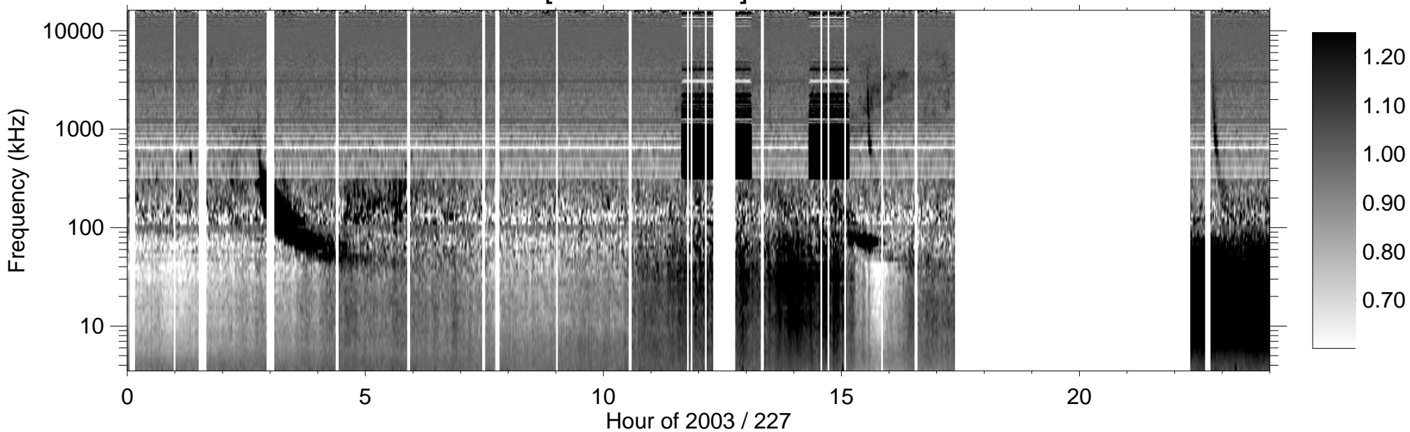
RPWS [ABCH1H2/Ex] (-B) 2003/08/15
