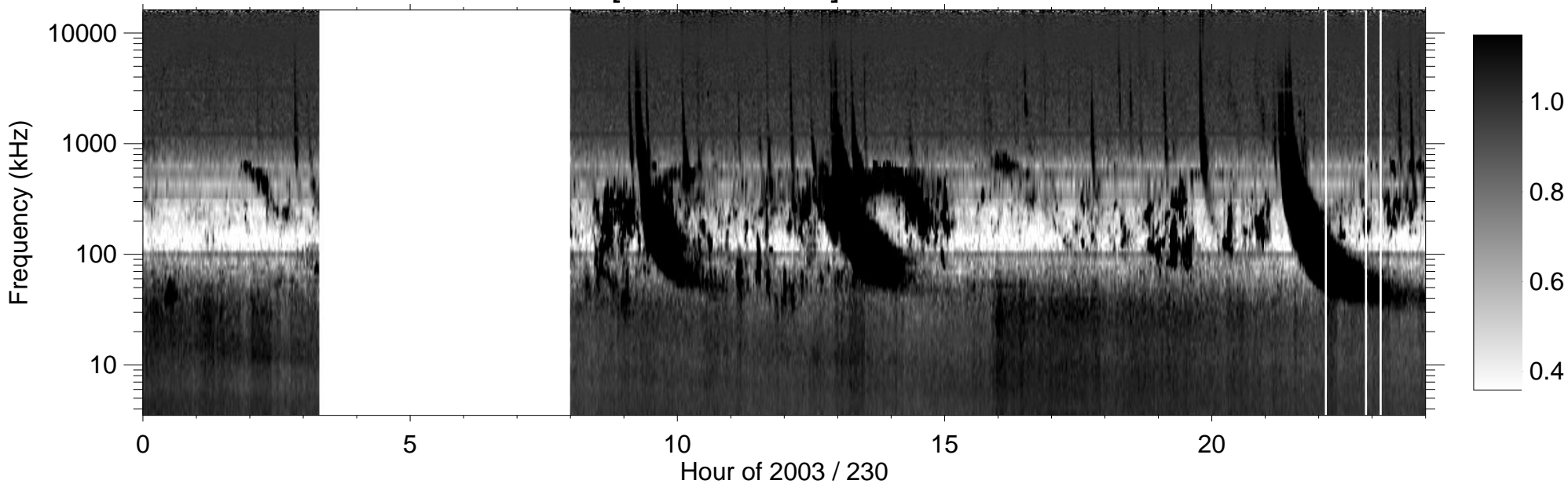
RPWS [ABCH1H2/Ex] (-B) 2003/08/18
