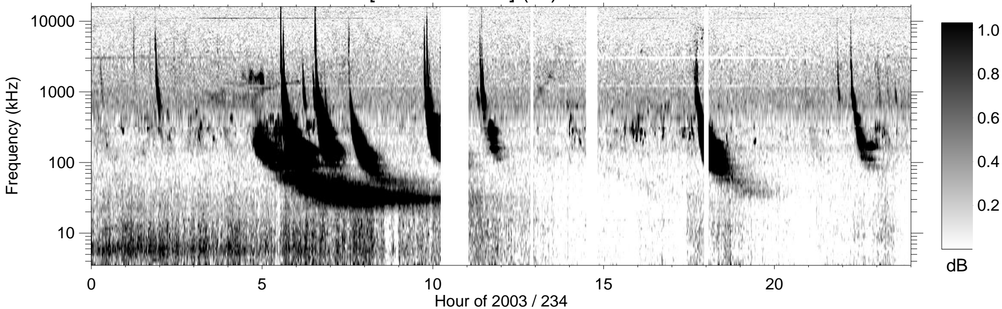
RPWS [ABCH1H2/Ex] (-B) 2003/08/22
