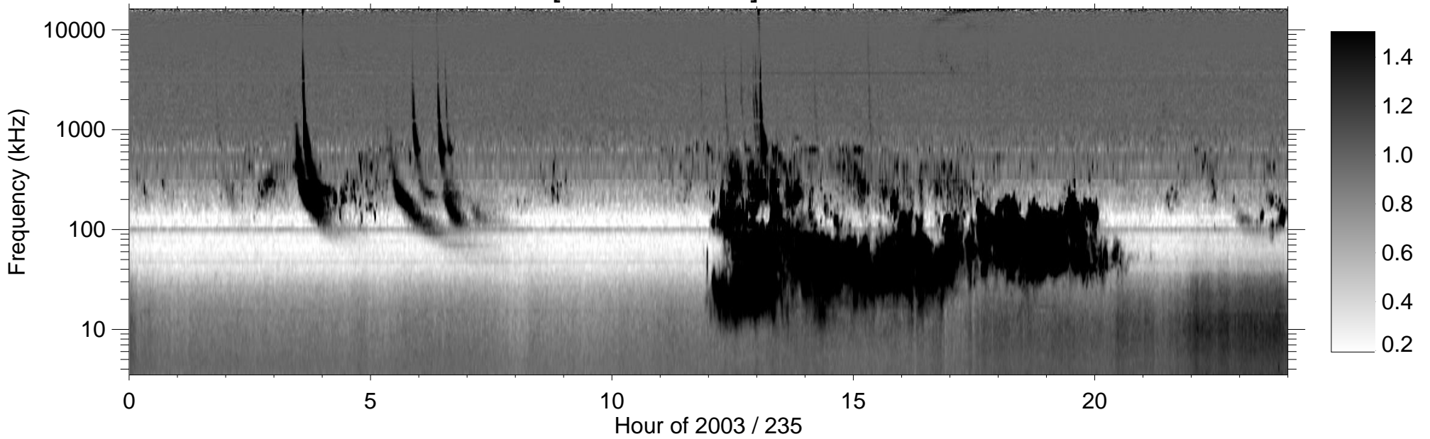
RPWS [ABCH1H2/Ex] (-B) 2003/08/23
