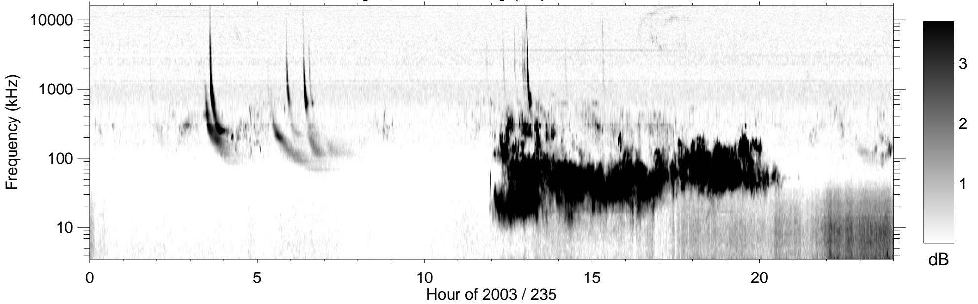
RPWS [ABCH1H2/Ex] (-B) 2003/08/23
