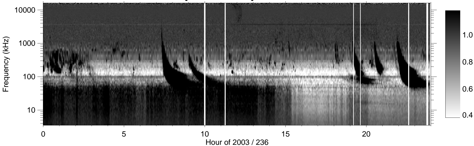
RPWS [ABCH1H2/Ex] (-B) 2003/08/24
