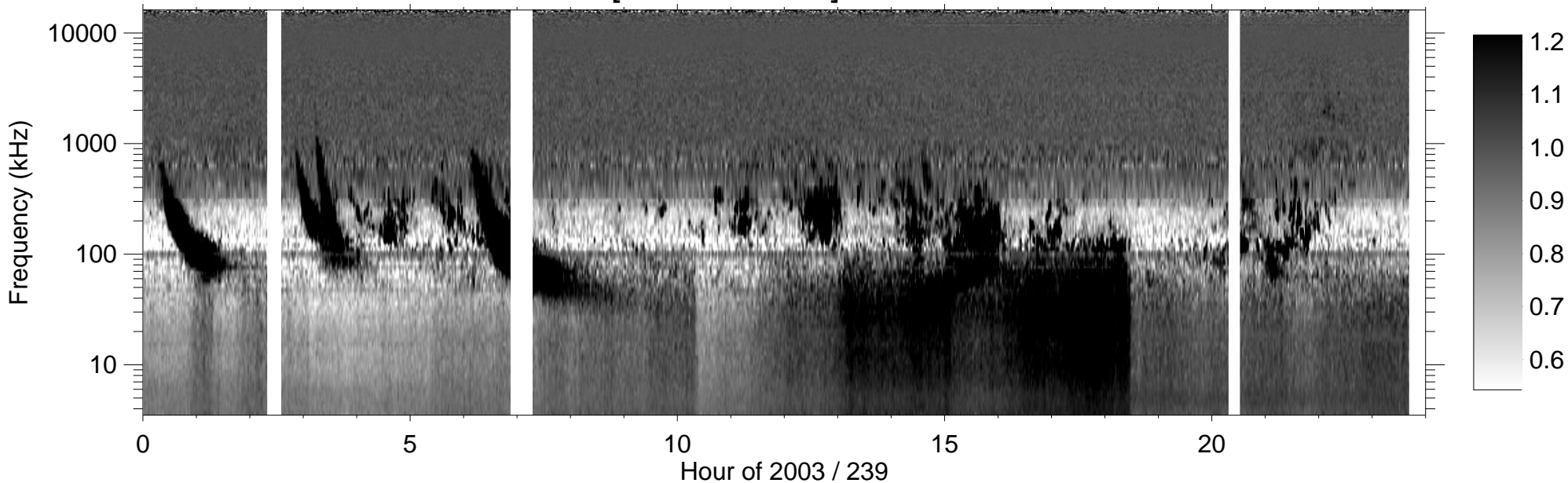
RPWS [ABCH1H2/Ex] (-B) 2003/08/27
