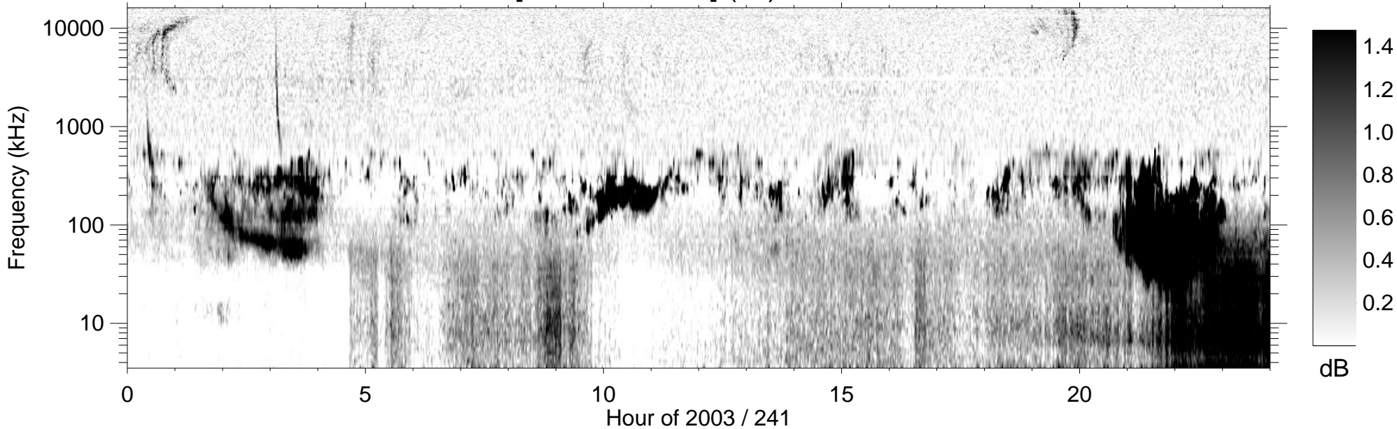
RPWS [ABCH1H2/Ex] (-B) 2003/08/29
