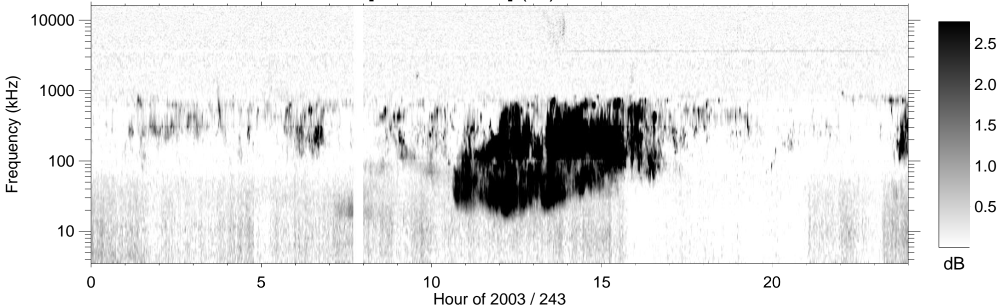
RPWS [ABCH1H2/Ex] (-B) 2003/08/31
